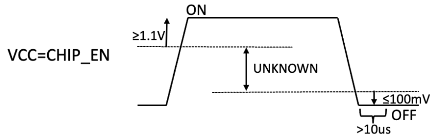
Figure 19. Power supply sequence when VCC=CHIP_EN (WLCSP10)
