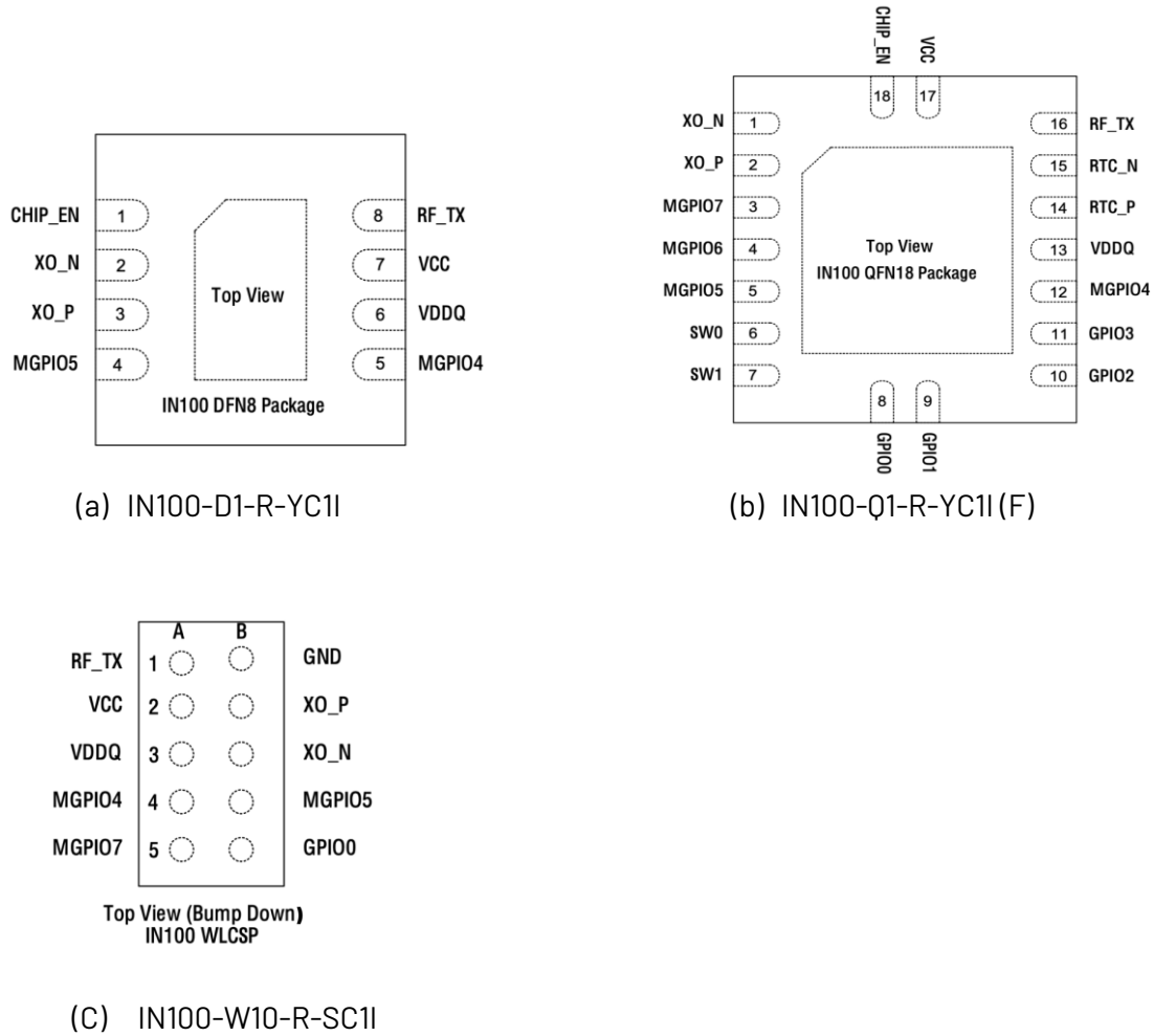
Figure 3 : Pin assignments
