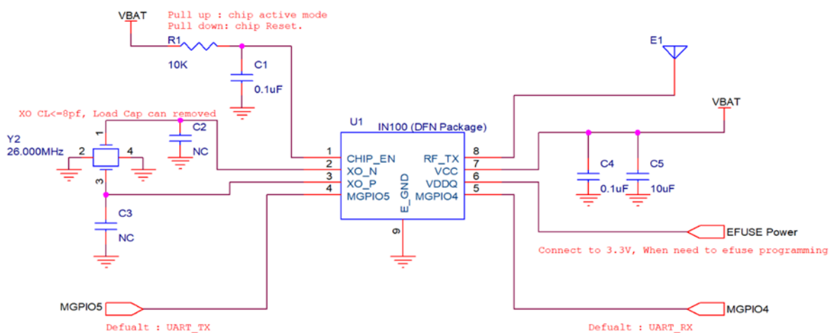
Figure 21 : IN100 DFN8 reference design
