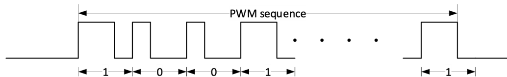
Figure 8 : PWM sequence
