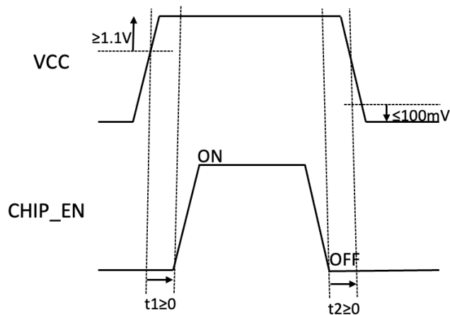
Figure 18 : Power supply sequence when VCC and CHIP_EN are separate (DFN8 or QFN18)
