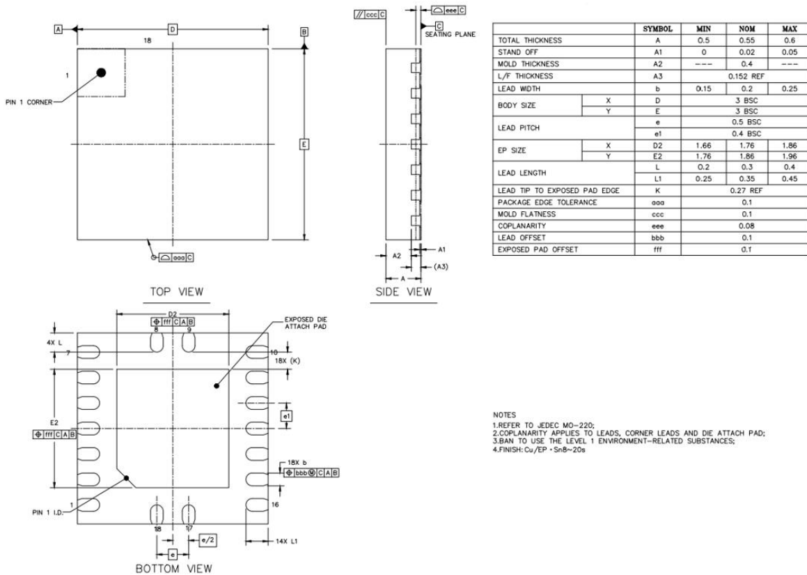
Figure 24 : QFN18 POD IN100-Q1-R-YC1I/ IN100-Q1-R-YC1F
