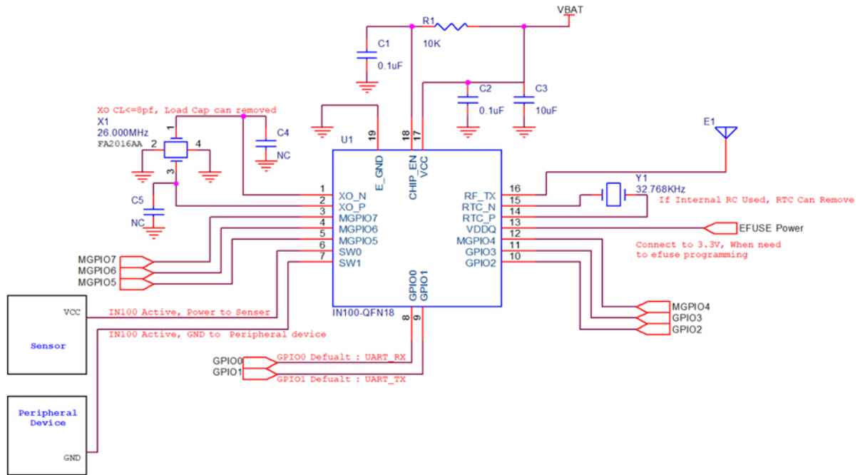
Figure 20 : IN100 QFN18 reference design
