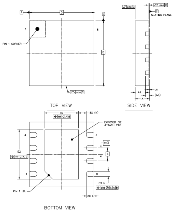
Figure 25 : DFN8 POD IN100-D1-R-YC1I
