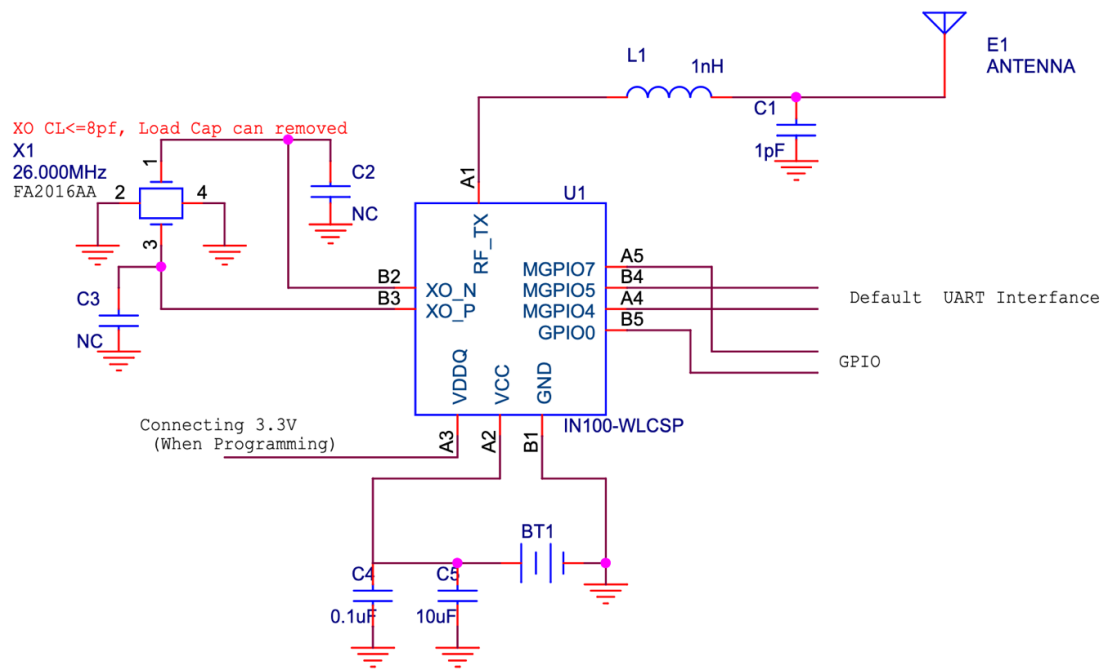
Figure 22 : IN100 WLCSP10 reference design
